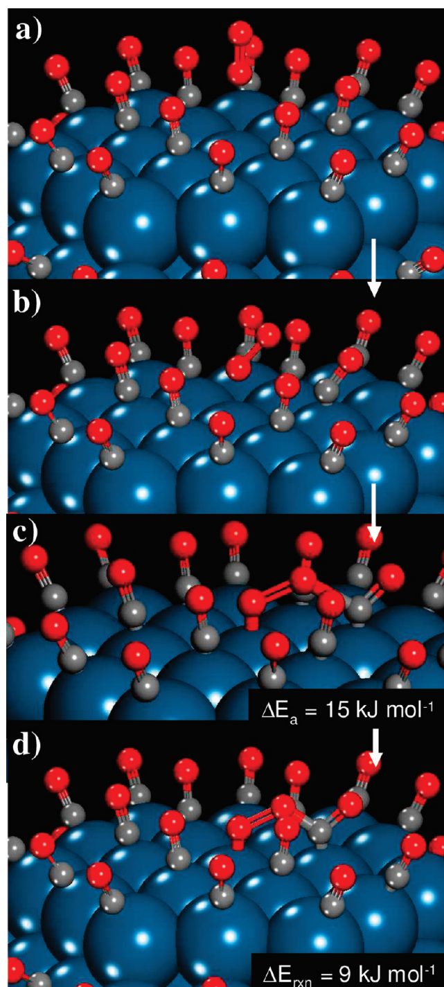
Figure 11. DFT-calculated reaction coordinate for the concerted reaction of O 2 (g) on the central vacant site on the (111) terrace on the fully CO covered Pt 201 cluster: (a) the reactant state (O 2 (g) + Pt 201 ), (b) an intermediate state along the coordinate, (c) the transition state, and (d) the final O*–O–C=O* state.
