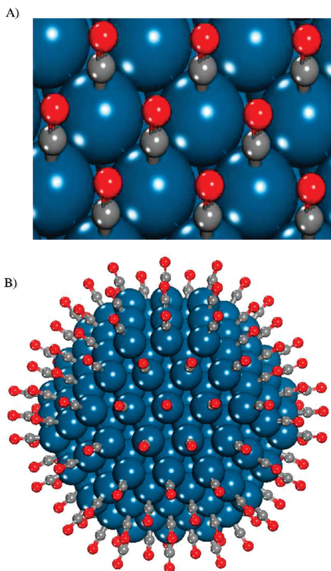
Figure 1. Structural models for (A) the Pt(111) surface and (B) small Pt particles ( \text{Pt}_{201} atom cluster).
