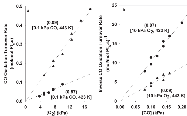
Figure 5. Effects of (a) O 2 pressure and (b) CO pressure on rates and inverse rates of CO oxidation, respectively, for Pt/Al 2 O 3 (0.87) at 423 K and Pt/Al 2 O 3 (0.09) at 443 K.
