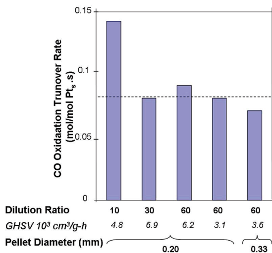
Figure 4. CO oxidation turnover rates for Pt/Al 2 O 3 (0.87) at 423 K (0.1 kPa CO, 0.2 kPa Ar, 10 kPa O 2 , balance He) measured at 10, 30, and 60 intrapellet dilution ratios and 0.2 mm and 0.33 mm pellet diameters ( 3.1 \times 10^3 – 6.9 \times 10^3 cm 3 /g-h space velocities).
