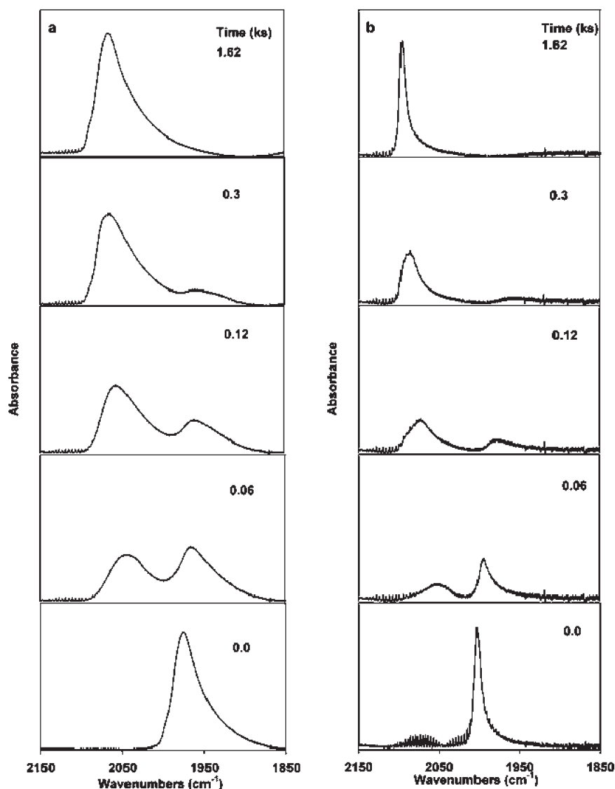
Figure 15. Infrared spectra during exchange between ^{12}\text{CO}(\text{g}) and chemisorbed ^{13}\text{CO}^* at 303 K for (a) \text{Pt}/\text{Al}_2\text{O}_3 (0.87) and (b) \text{Pt}/\text{Al}_2\text{O}_3 (0.05).
