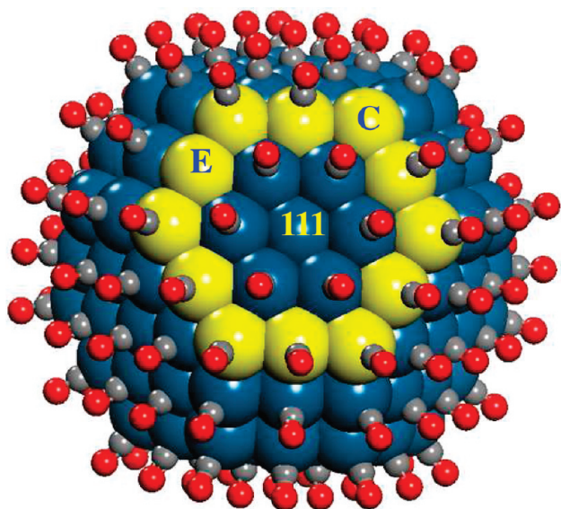
Figure 10. Different vacancy sites on the fully CO covered Pt 201 cuboctahedral cluster examined theoretically. The 111 terrace, edge, and corner sites labeled have coordination numbers of 9, 7, and 6, respectively.
